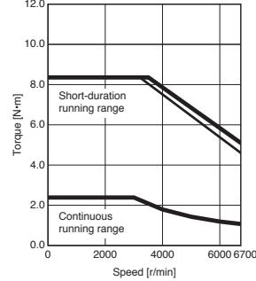
HK-KT7M3W Standard torque
