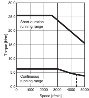
HK-KT203W Torque increased
