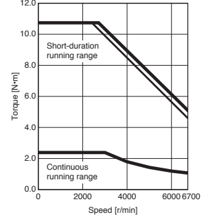
HK-KT7M3W Torque increased
