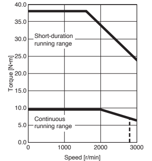
HK-KT202W Torque increased
