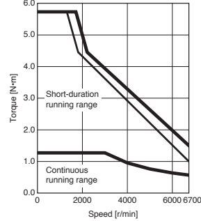
HK-KT43UW Torque increased
