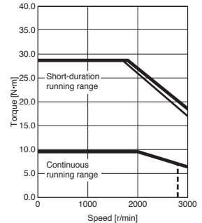
HK-KT202W Standard torque
