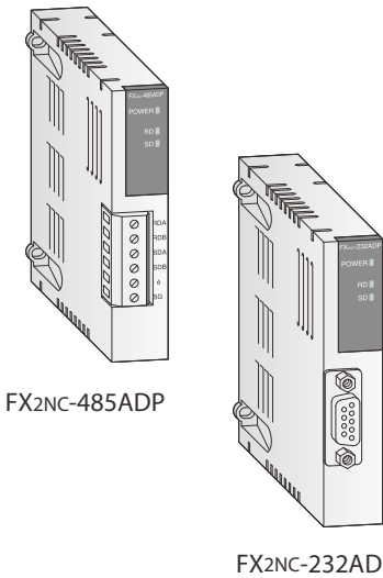
FX2NC-232ADP
